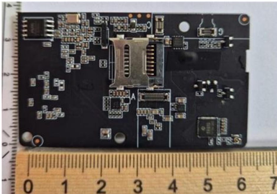
Mainboard
