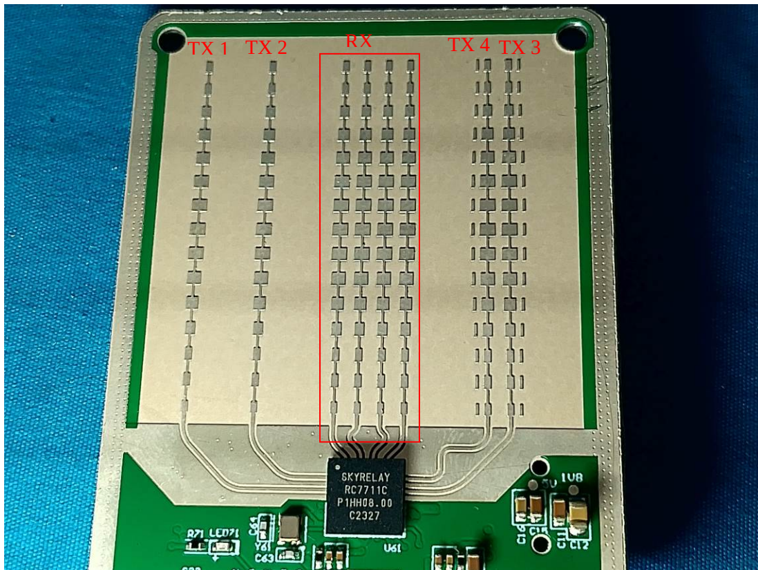
Radar Antenna
