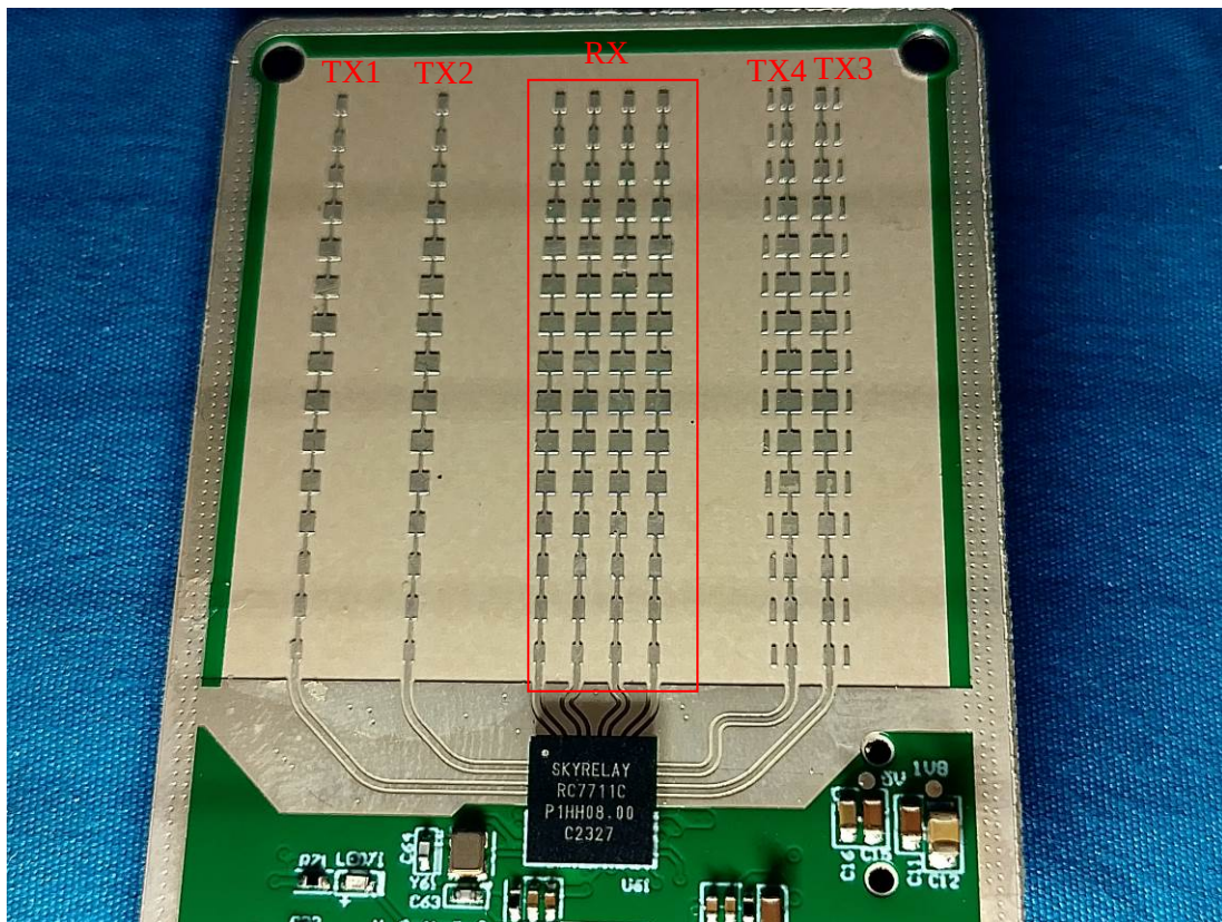
Radar Antenna
