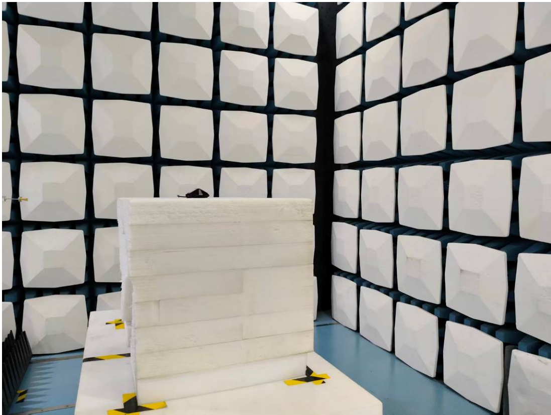
Radiated Emission 220-231GHz View
