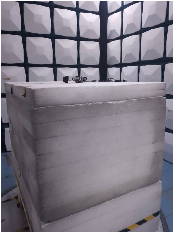
Radiated Emission 90-140GHz View
