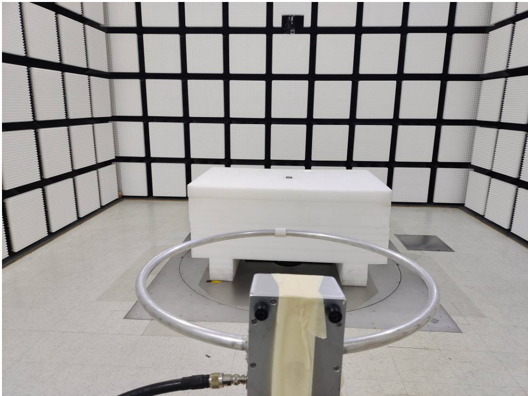
Radiated Emissio 9kHz-30MHz View-Ground-parallel
