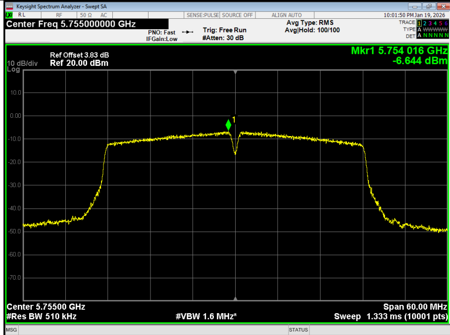
Power_Spectral_Density_NVNT_ANT1_802_11ac(VHT40)_5755
