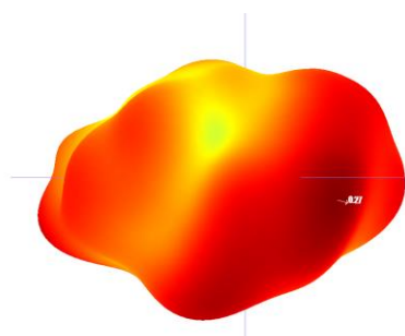
DCS1800/LTE B3/6E
