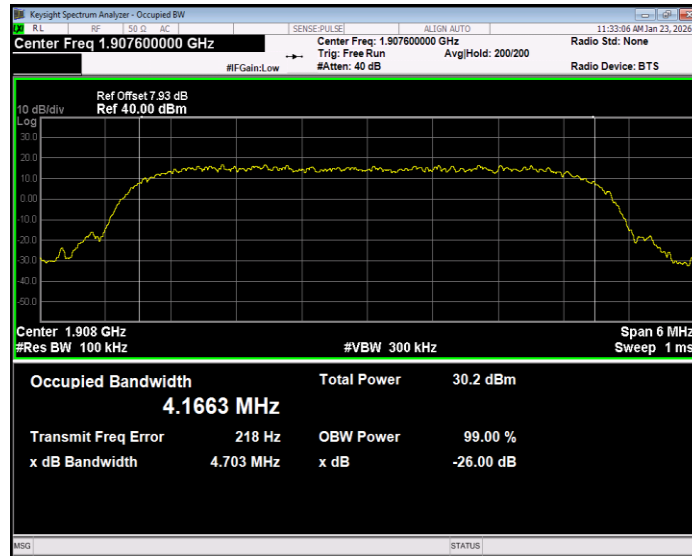
WCDMA Band5 Channel=4132
