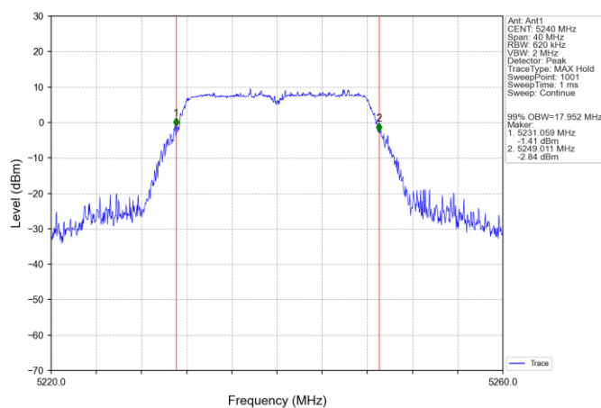
802.11a_HCH_5240MHz_Ant1_NTNV
