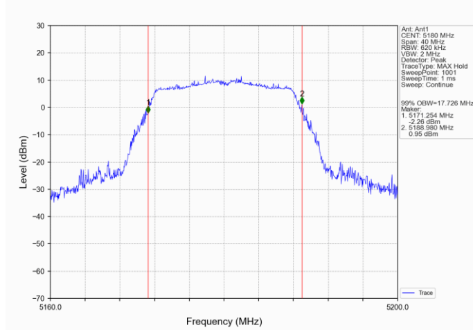
802.11a_LCH_5180MHz_Ant1_NTNV
