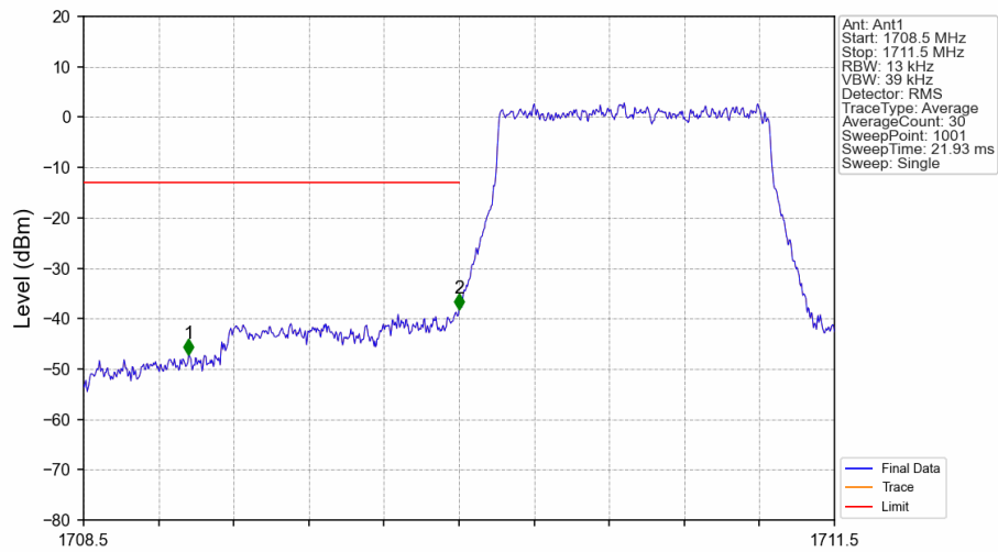
Band66_1.4MHz_QPSK_LCH_1710.7MHz_RB_6_0_NTNV
