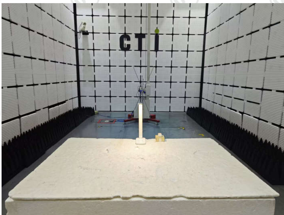
Radiated Emissions Test Setup-2 (30MHz-1GHz)
