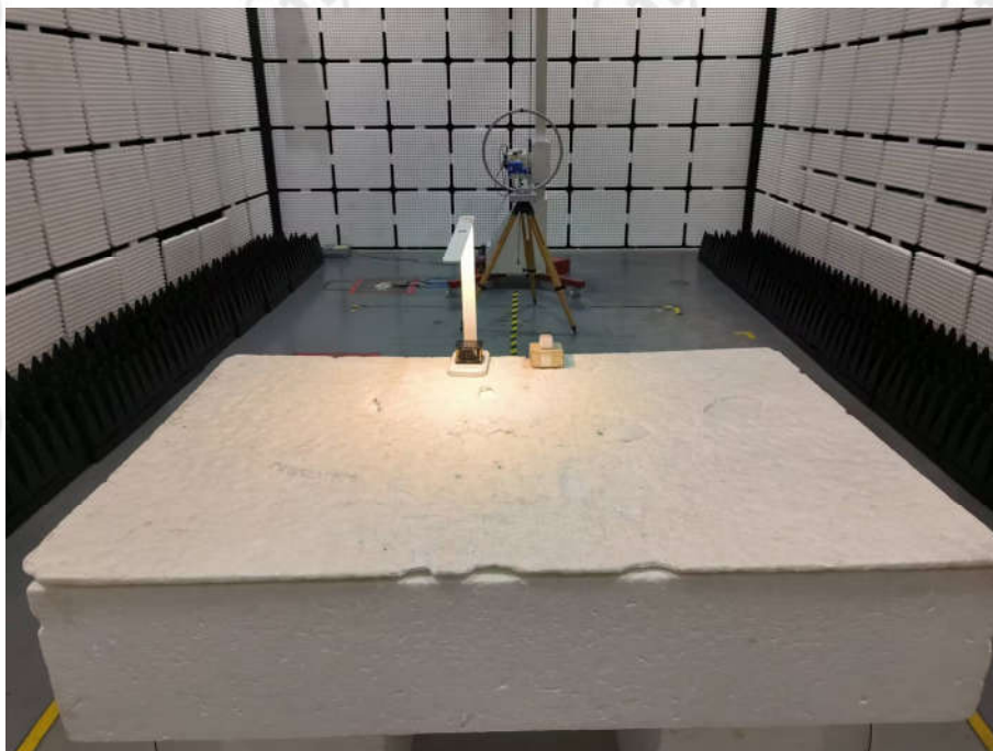
Radiated Emissions Test Setup-1 (9kHz-30MHz)
