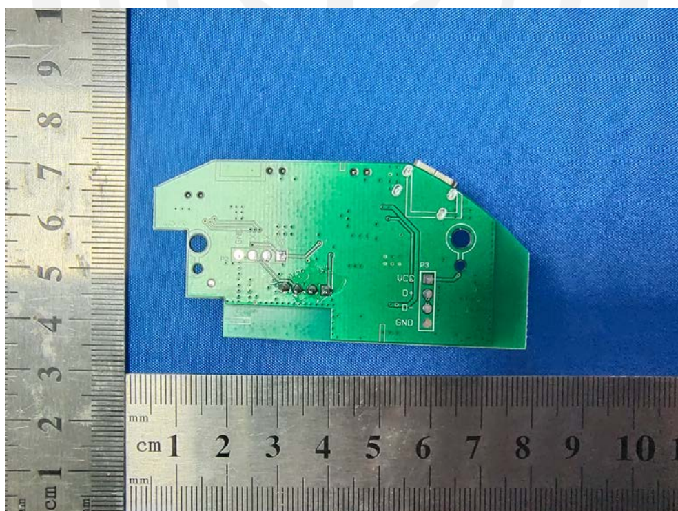
Antenna1 BT Antenna location
