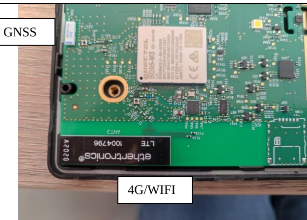
GNSS / LTE / WIFI antennas
