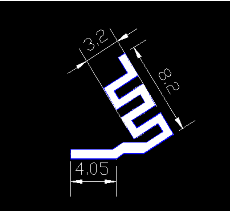
Antenna Photo & Length(mm)
