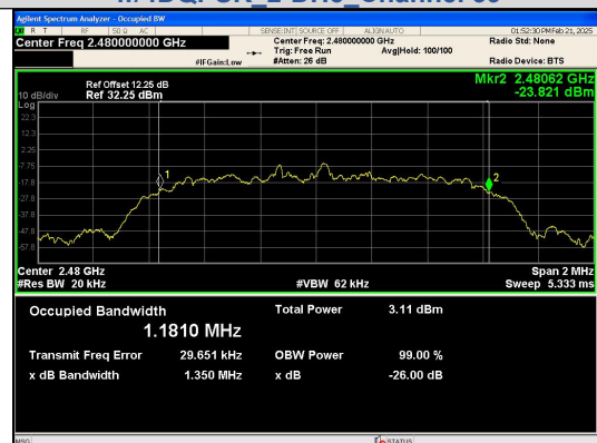
π/4DQPSK 2-DH5 Channel 78
