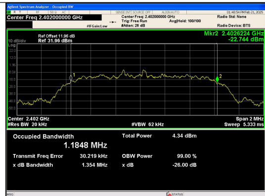
π/4DQPSK_2-DH5_Channel 0
