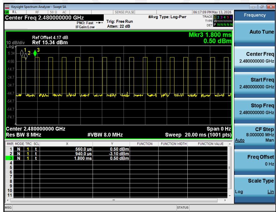
Duty_Cycle_NVNT_ANT1_1-DH1_2480
