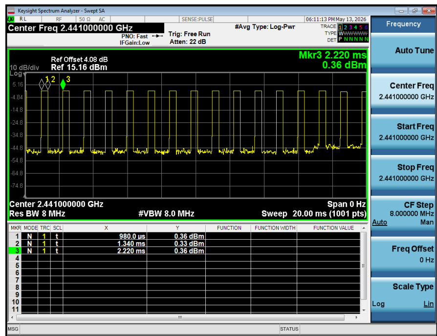
Duty_Cycle_NVNT_ANT1_1-DH1_2441
