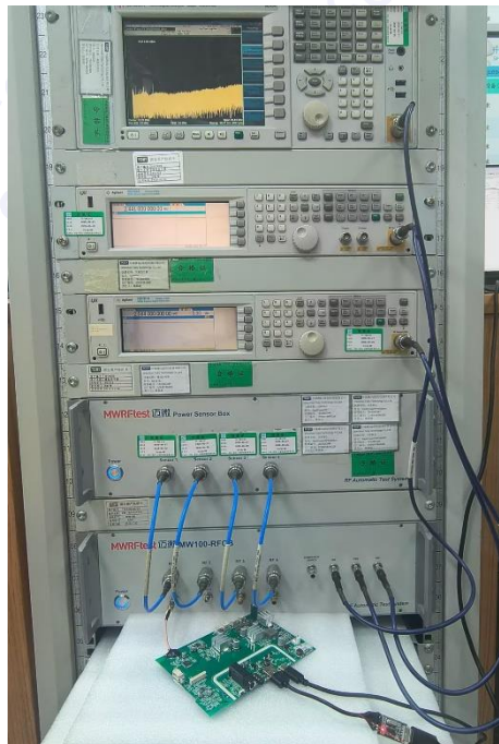
Photo of Setup for Conducted Measurements
