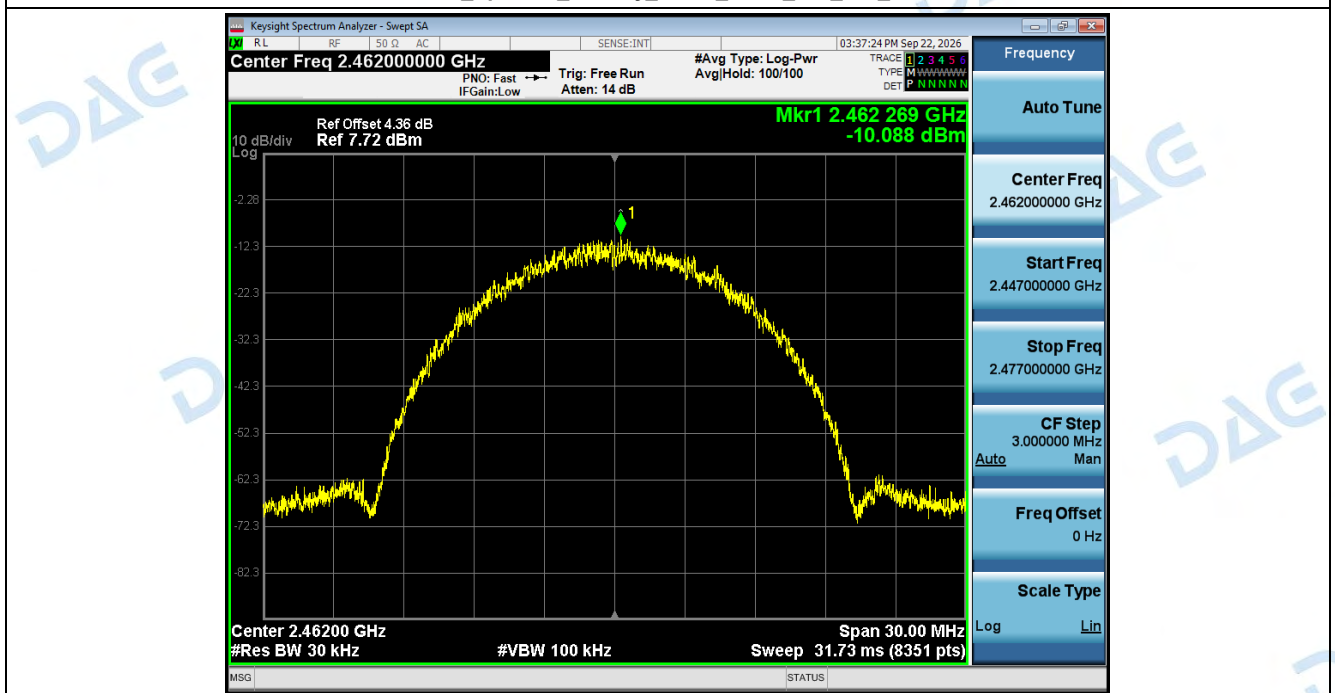
Power_Spectral_Density_NVNT_ANT1_802_11b_2462
