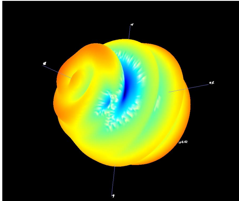
B1.1 3D Pattern for 430MHz
