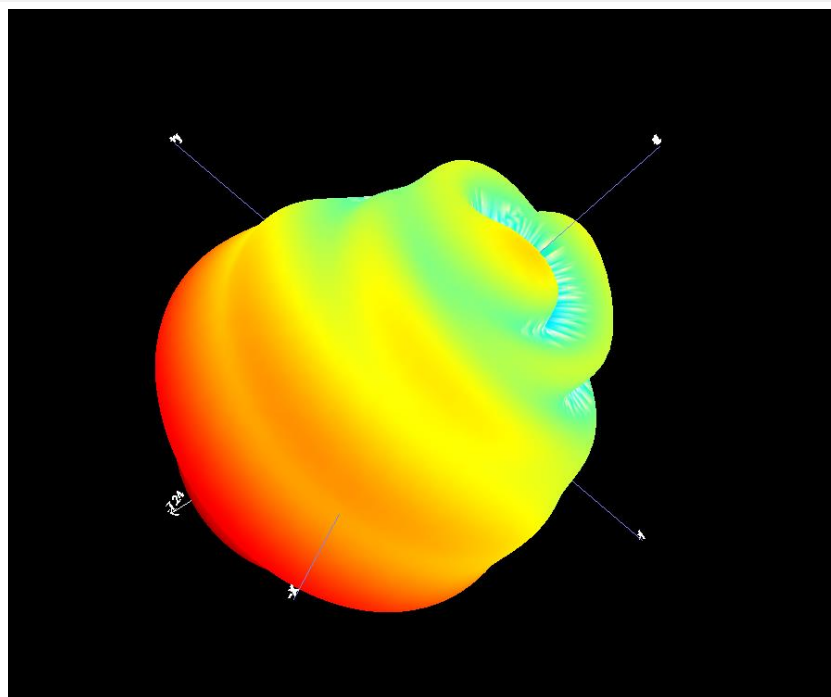
B1.3 3D Pattern for 450MHz
