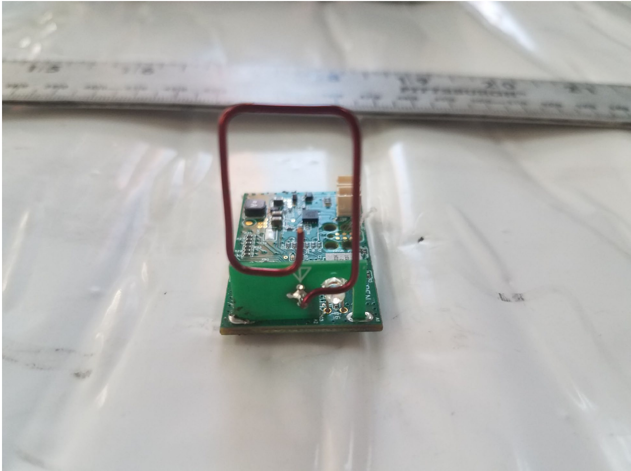
Figure 8. Antenna
