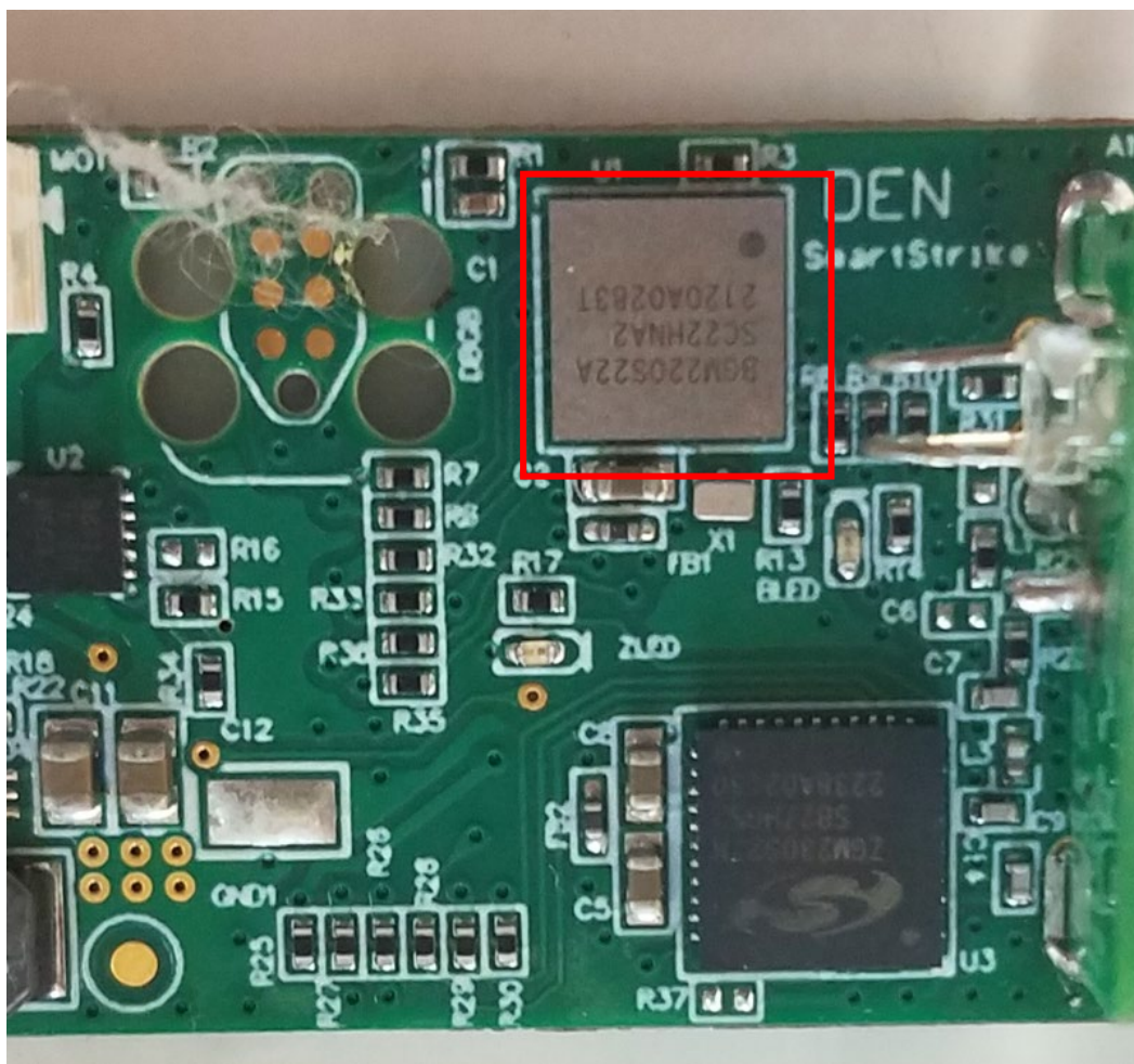
Figure 6. BLE SIP module. Internal antenna used.
