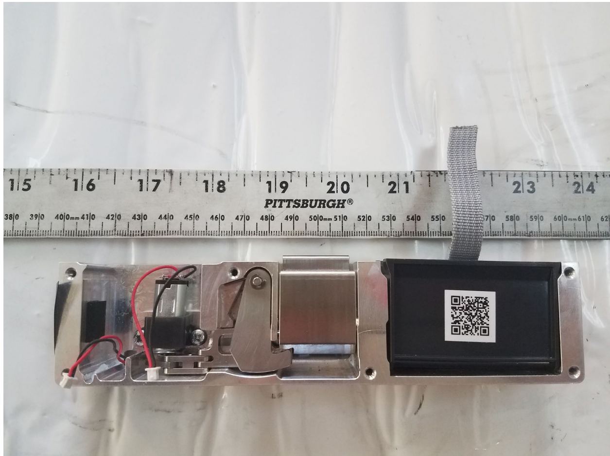
Figure 3. PCBA removed
