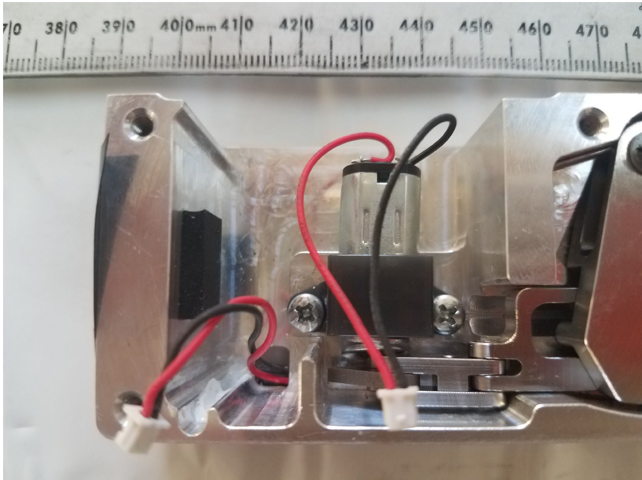
Figure 4. Motor assembly
