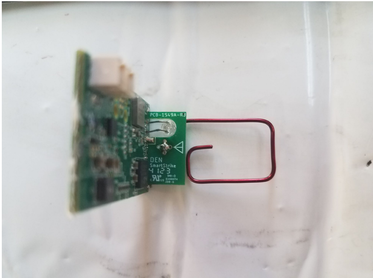
Figure 7. Secondary PCBA
