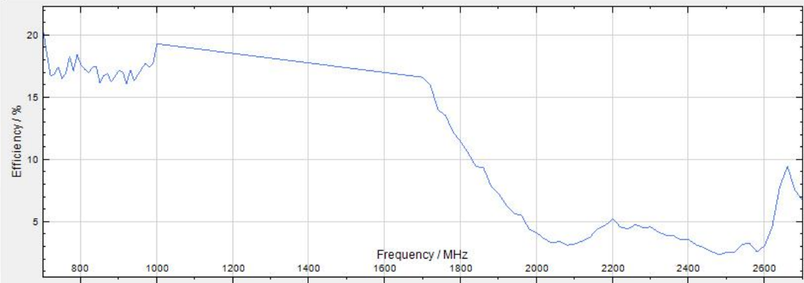
700M-2700MEfficiency%
