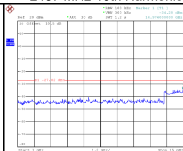
2437 MHz-10th Harmonics
