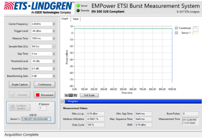
Figure 8.4-5: Maximum peak output power, GFSK, 2 Mbps, 2440 MHz
