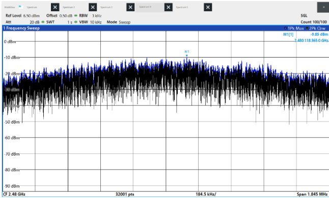
Figure 8.6-6: Power spectral density, GFSK, 2 Mbps, 2480 MHz
