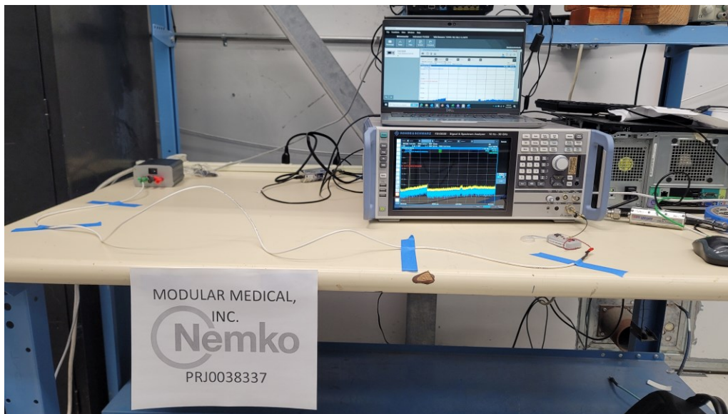
Figure 16 – Spectrum analyzer setup.
