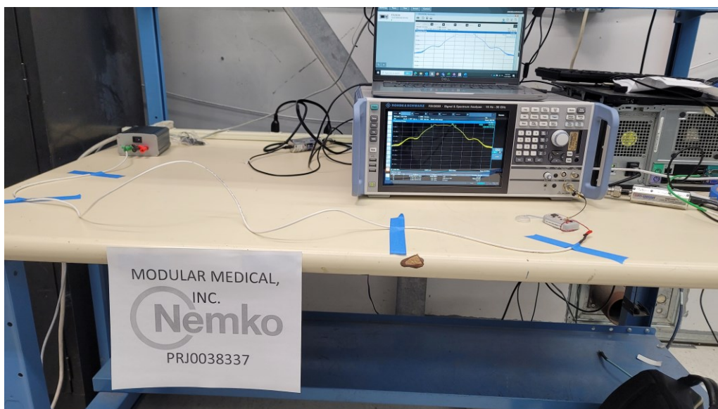
Figure 15 – Spectrum analyzer setup.
