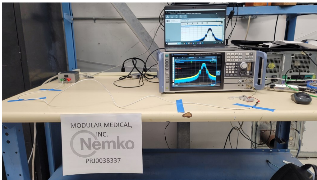
Figure 17 – Spectrum analyzer setup.
