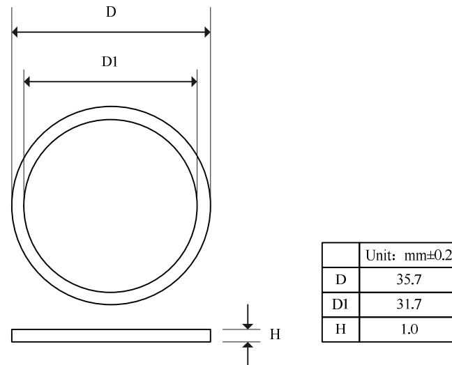
Figure 1. Dimensions
