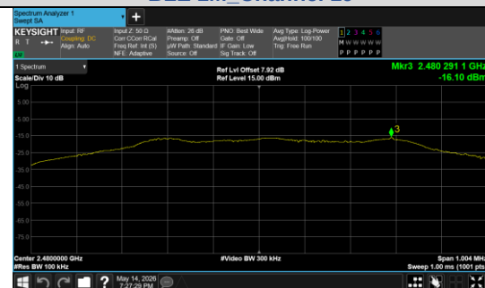
In-Band Reference Level BLE 1M_Channel 39
