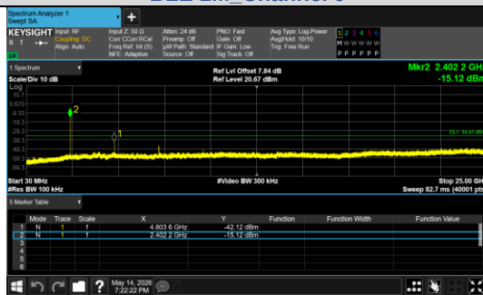
30.0 MHz - 25000.0 MHz BLE 1M_Channel 0
