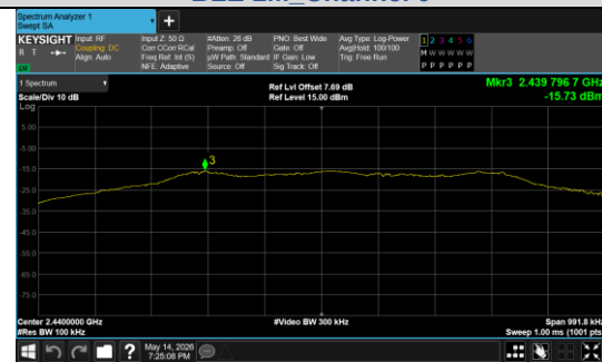
In-Band Reference Level BLE 1M_Channel 19
