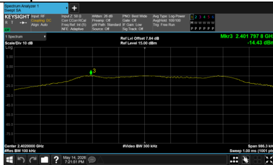
In-Band Reference Level BLE 1M_Channel 0
