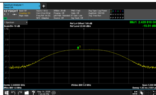
Peak Output Power BLE 1M_Channel 19
