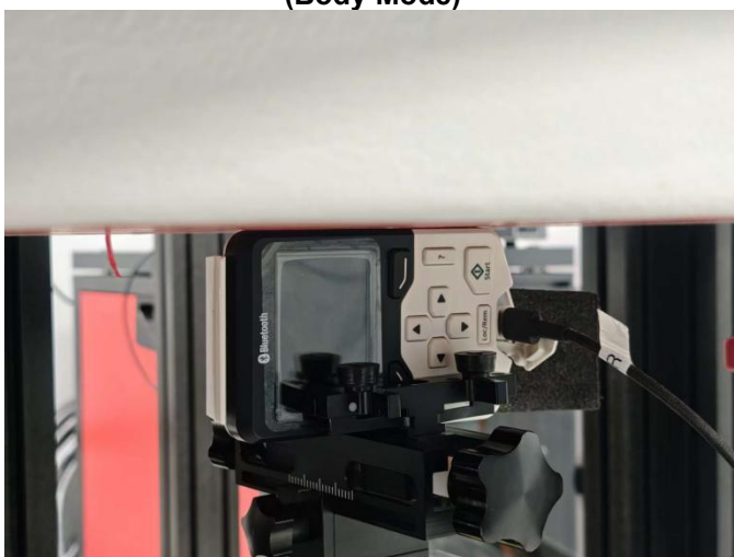
Right Side of EUT with 0cm Gap (Body Mode)
