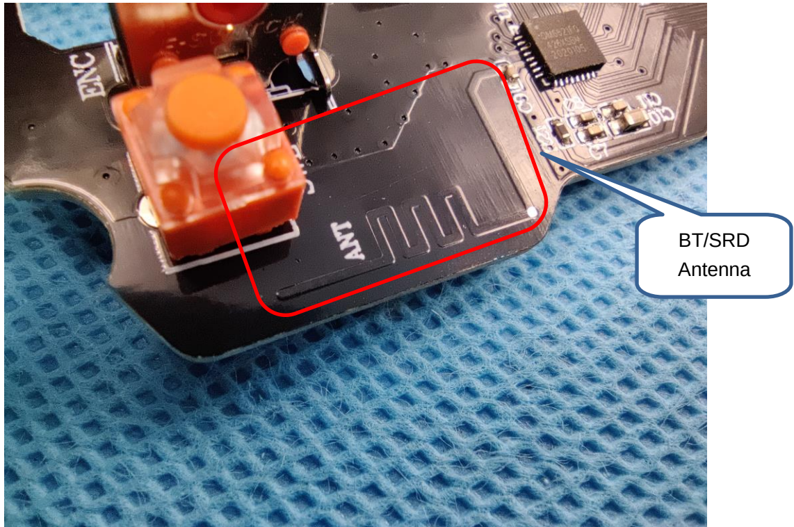
Internal view-4 of EUT
