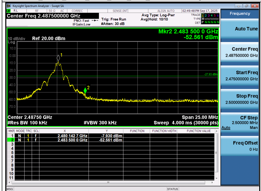
Test_Graph_GFSK_ANT1_2480_SRD_Higher Band Edge Emissions
