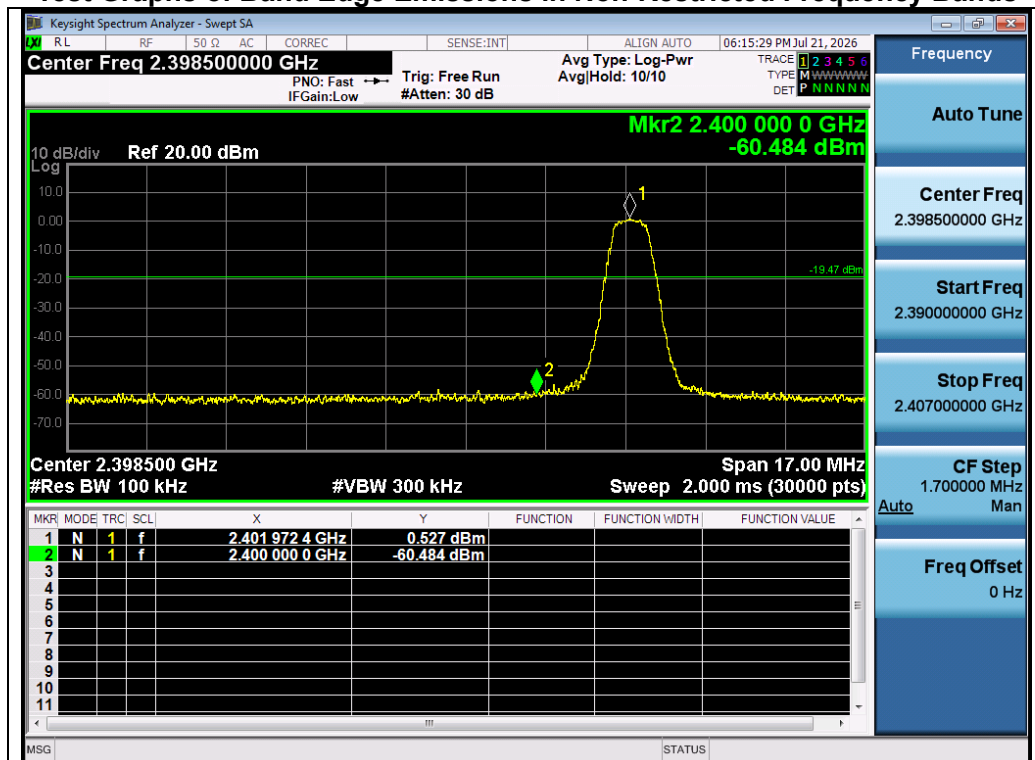
Test_Graph_2.4G_GFSK_ANT1_2402_Lower Band Edge Emissions
