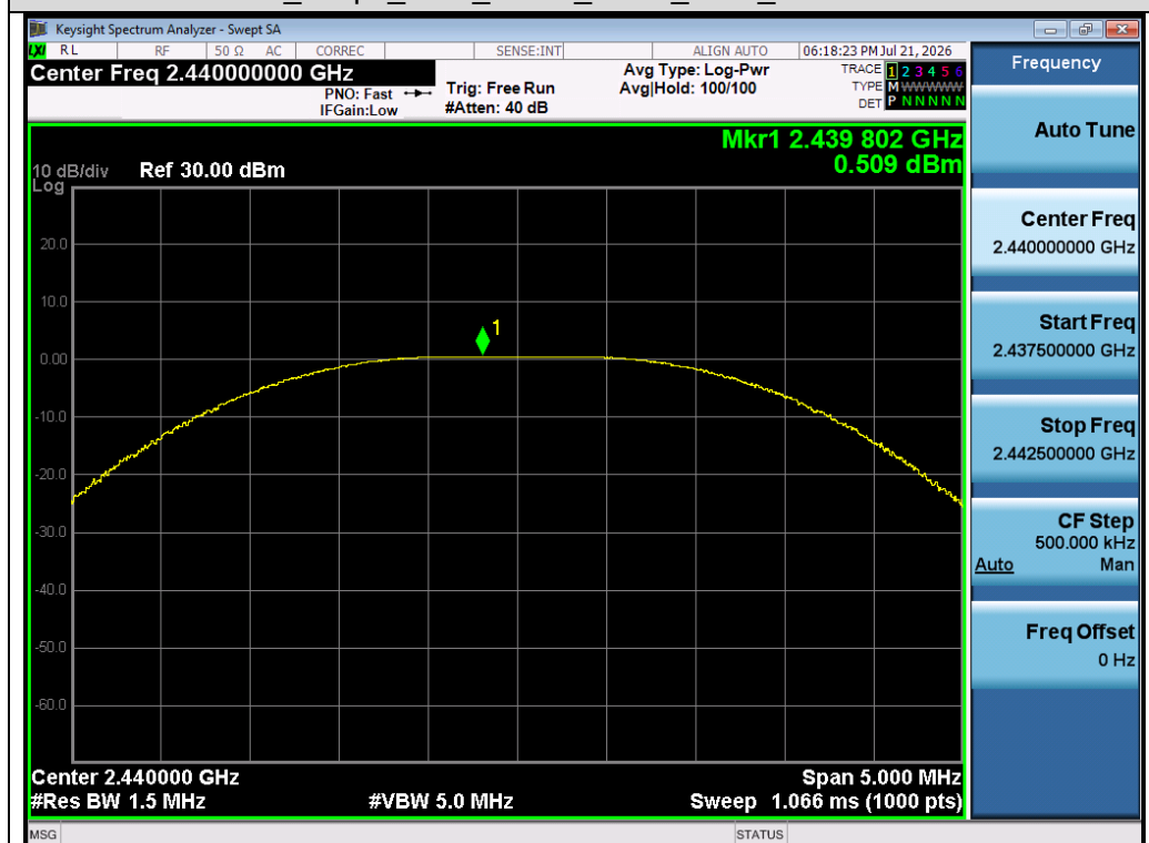
Test_Graph_2.4G_GFSK_ANT1_2440_Peak Power
