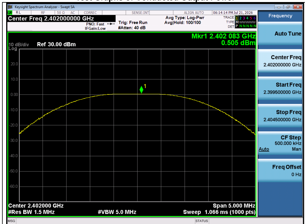
Test_Graph_2.4G_GFSK_ANT1_2402_Peak Power
