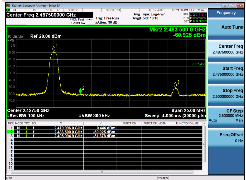
Test_Graph_2.4G_GFSK_ANT1_2480_Higher Band Edge Emissions
