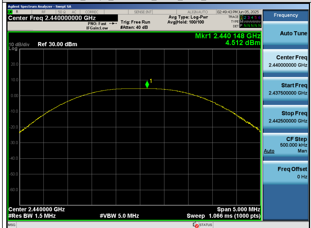
Test_Graph_SRD 2.4G_ANT1_2440_Peak Power
