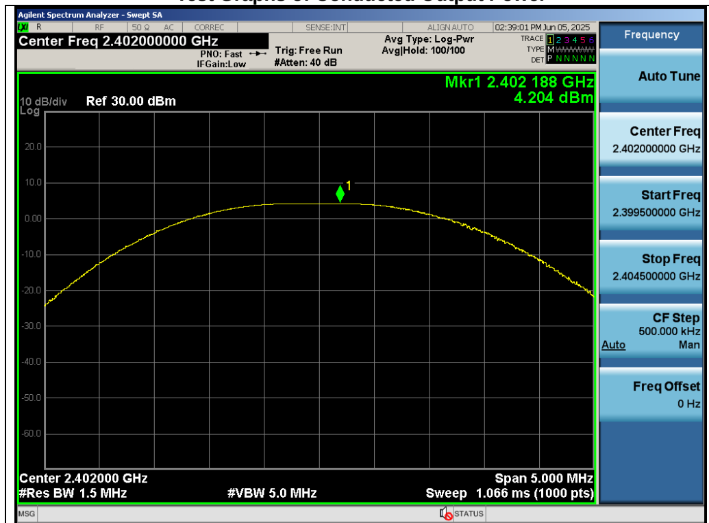
Test_Graph_SRD 2.4G_ANT1_2402_Peak Power
