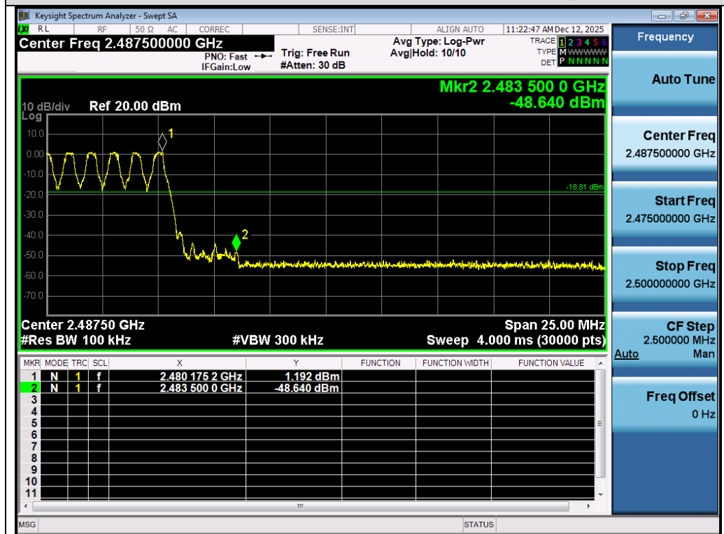
Test_Graph_2.4G_HOP_ANT1_NA_GFSK_Higher Band Edge Emissions
