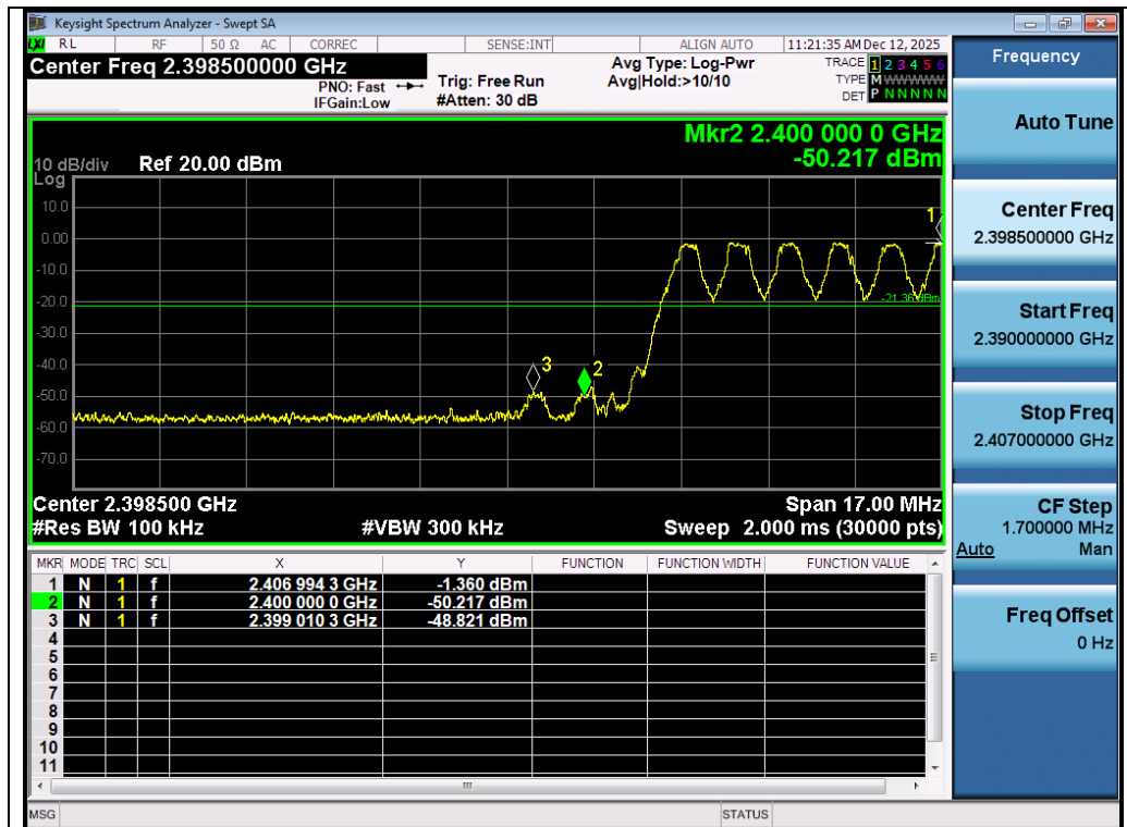
Test_Graph_2.4G_HOP_ANT1_NA_GFSK_Lower Band Edge Emissions
