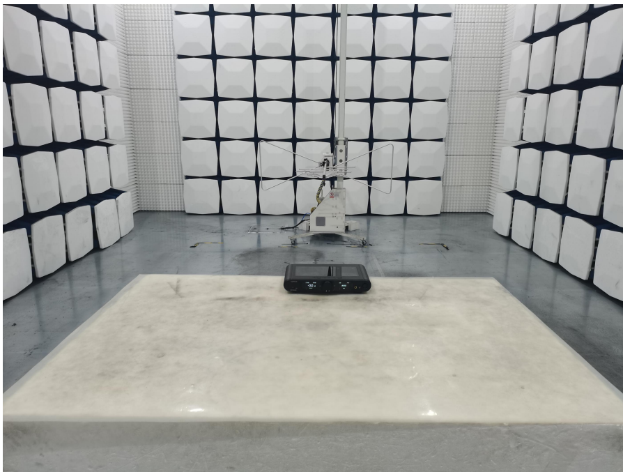
Radiated disturbance
