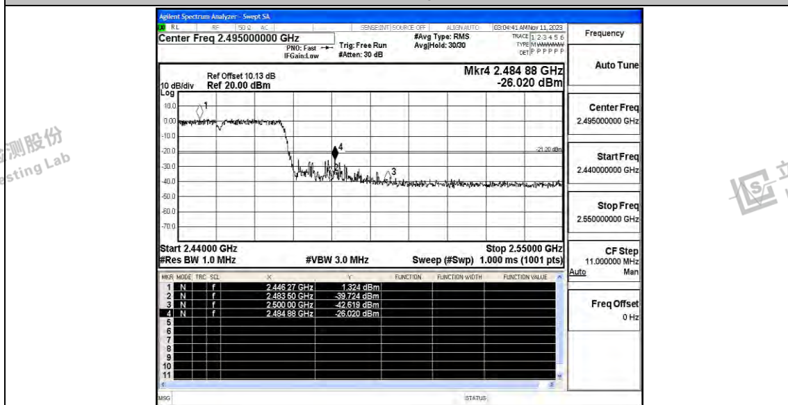
11N40SISO_mimo_High_2452_Peak
