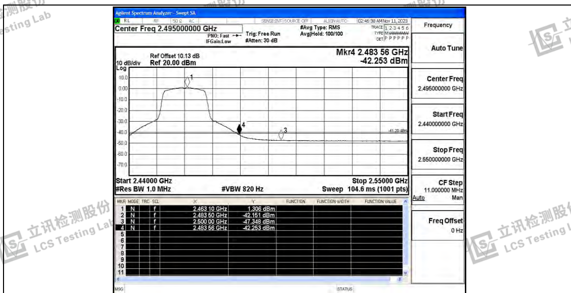
11G_Ant0_High_2462_Peak
