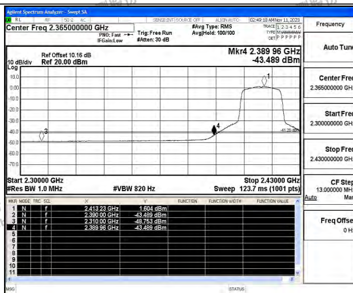
11N20SISO_mimo_Low_2412_Peak
