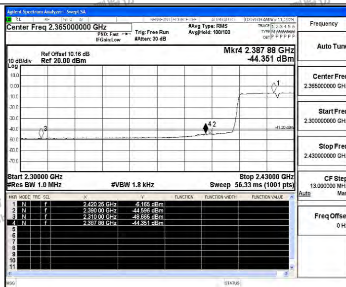
11N40SISO_mimo_Low_2422_Peak
