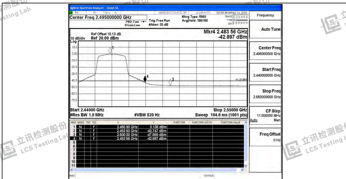
11N20SISO_mimo_High_2462_Peak
