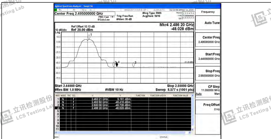
11B_Ant0_High_2462_Peak
