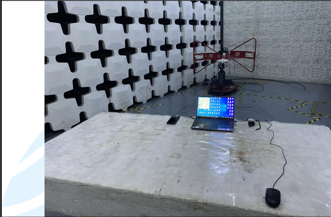
Radiated emission Test Setup (30 MHz~1 GHz) _Test Mode 7
