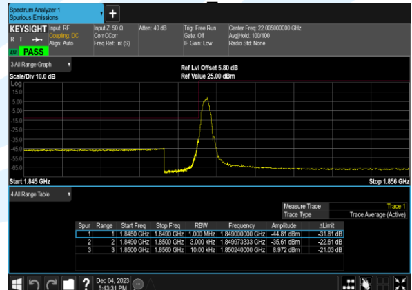
EGPRS1900_Channel512
