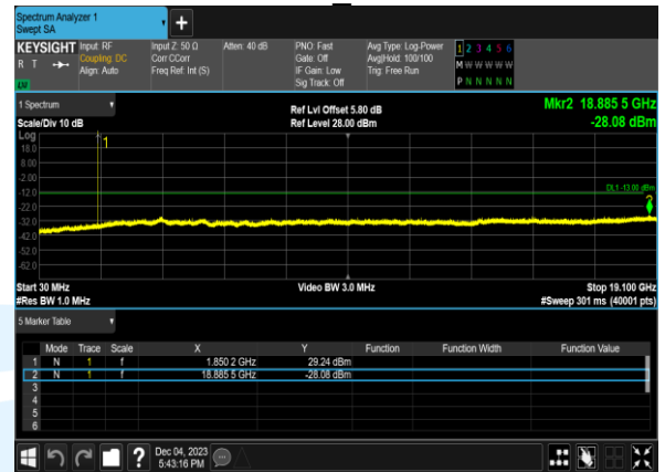
EGPRS1900 Channel512
