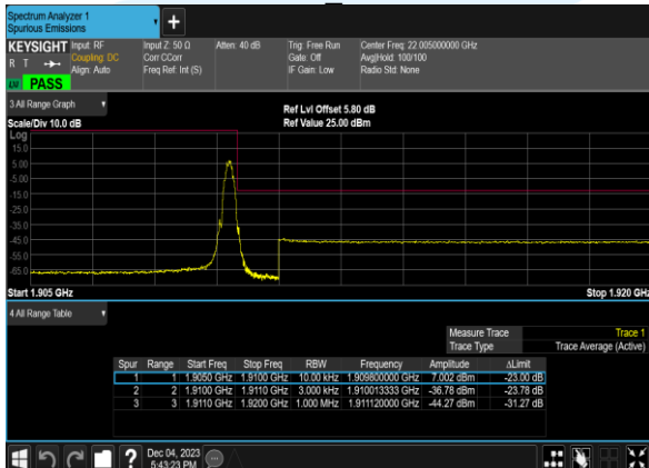
EGPRS1900_Channel810
