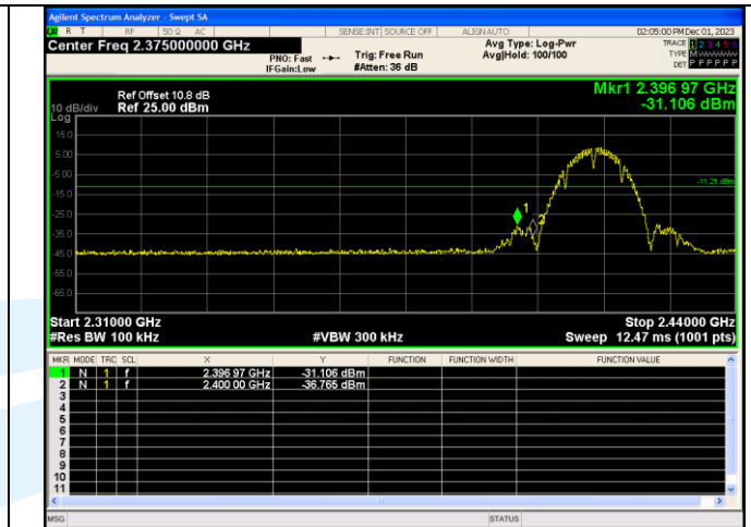
Out Of Band Emission IEEE 802.11b Channel 1 20MHz
