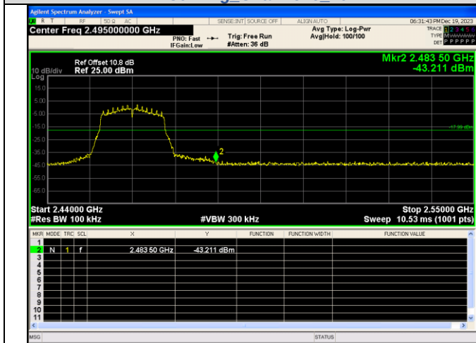
Out Of Band Emission IEEE 802.11g Channel 11 20MHz
