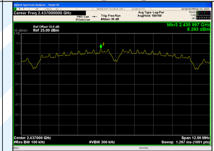
In-Band Reference Level IEEE 802.11b Channel 6 20MHz
