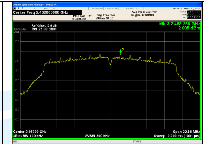
In-Band Reference Level IEEE 802.11g Channel 11 20MHz
