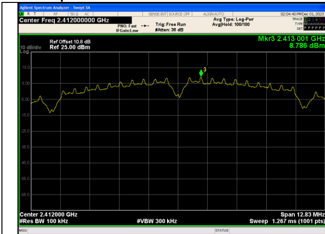
In-Band Reference Level IEEE 802.11b Channel 1 20MHz
