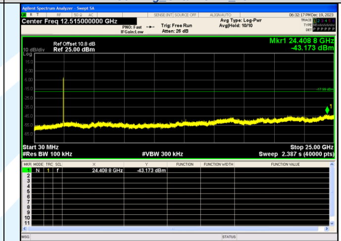
Spurious Emission IEEE 802.11g Channel 11 20MHz
