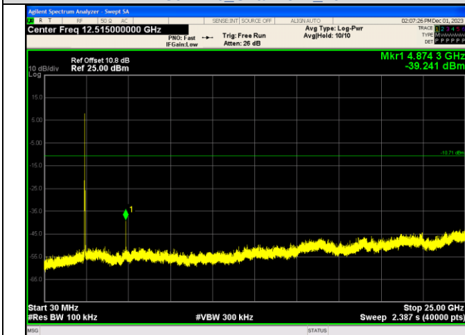
Spurious Emissions IEEE 802.11b Channel 6 20MHz
