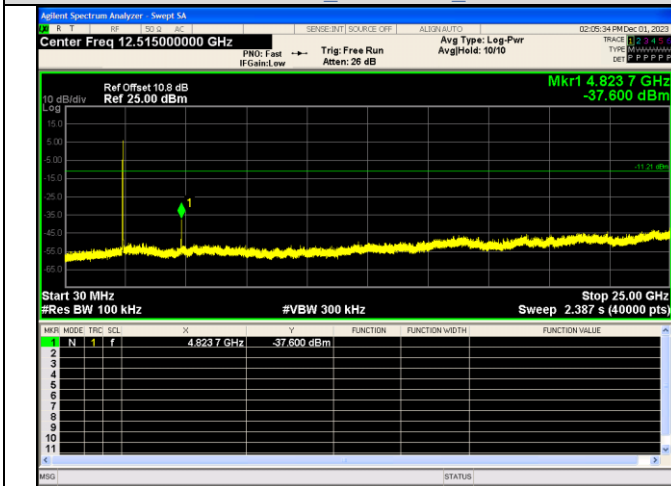
Spurious Emission IEEE 802.11b Channel 1 20MHz
