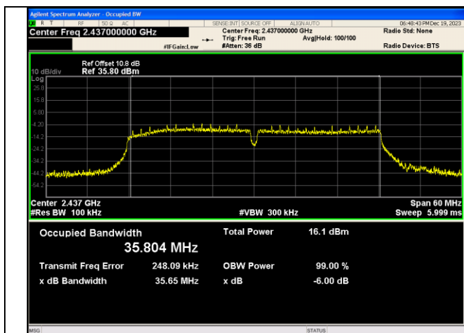
IEEE 802.11n Channel 6 40MHz
