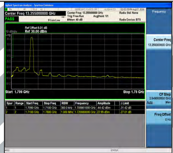
66C-10MHz-20MHz-QPSK@QPSK-QPSK@QPSK- 132027-132171-1RB#49@50RB#0-0RB#0@100RB#0- PASS
