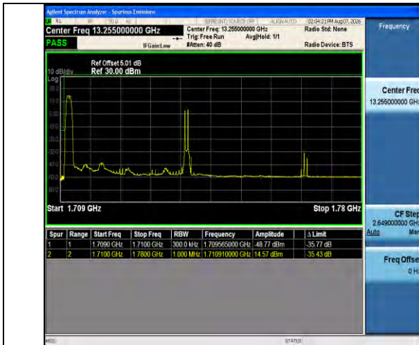
66C-10MHz-20MHz-QPSK@QPSK-QPSK@QPSK- 132027-132171-1RB#0@50RB#0-1RB#99@100RB#0- PASS
