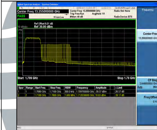
66C-10MHz-20MHz-QPSK@QPSK-QPSK@QPSK- 132027-132171-50RB#0@50RB#0-100RB#0@100RB#0- PASS
