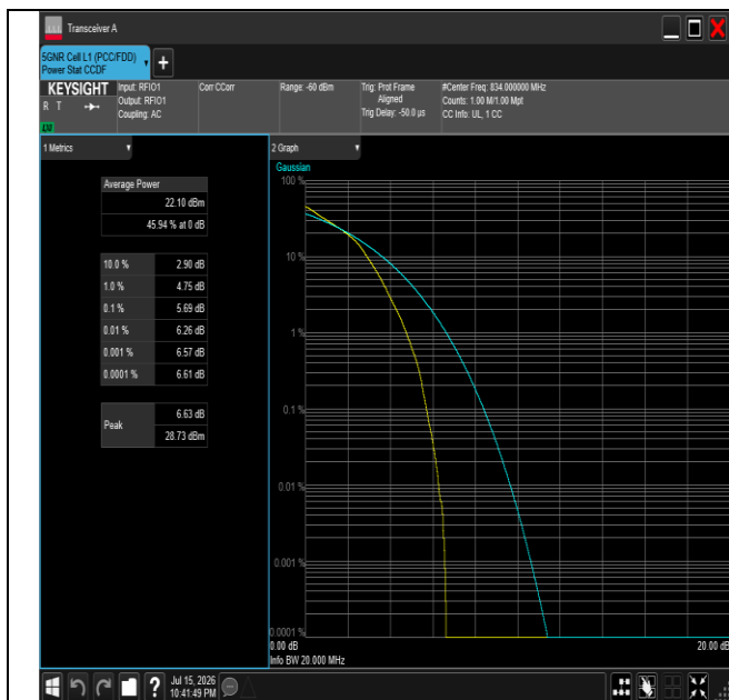
NTNV-n26(824-849)-PC3-15-20-L-DFT-16QAM-Outter_Full-P ASS
