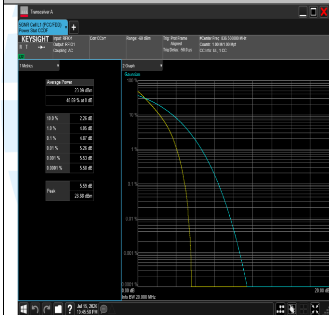
NTNV-n26(824-849)-PC3-15-20-M-DFT-QPSK-Outter_Full-P ASS
