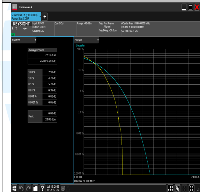
NTNV-n26(824-849)-PC3-15-20-H-DFT-16QAM-Outter_Full-P
