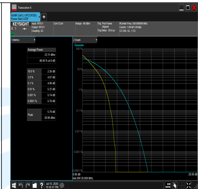
NTNV-n26(824-849)-PC3-15-20-H-DFT-QPSK-Outter_Full-PA
