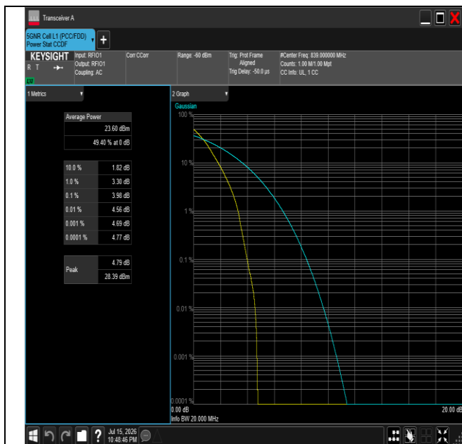
NTNV-n26(824-849)-PC3-15-20-H-DFT-BPSK-Outter_Full-PA
