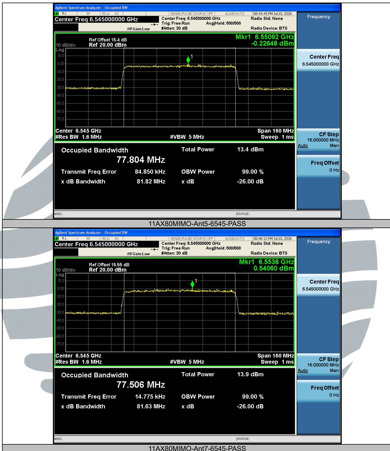
11AX80MIMO-Ant7-6545-PASS
