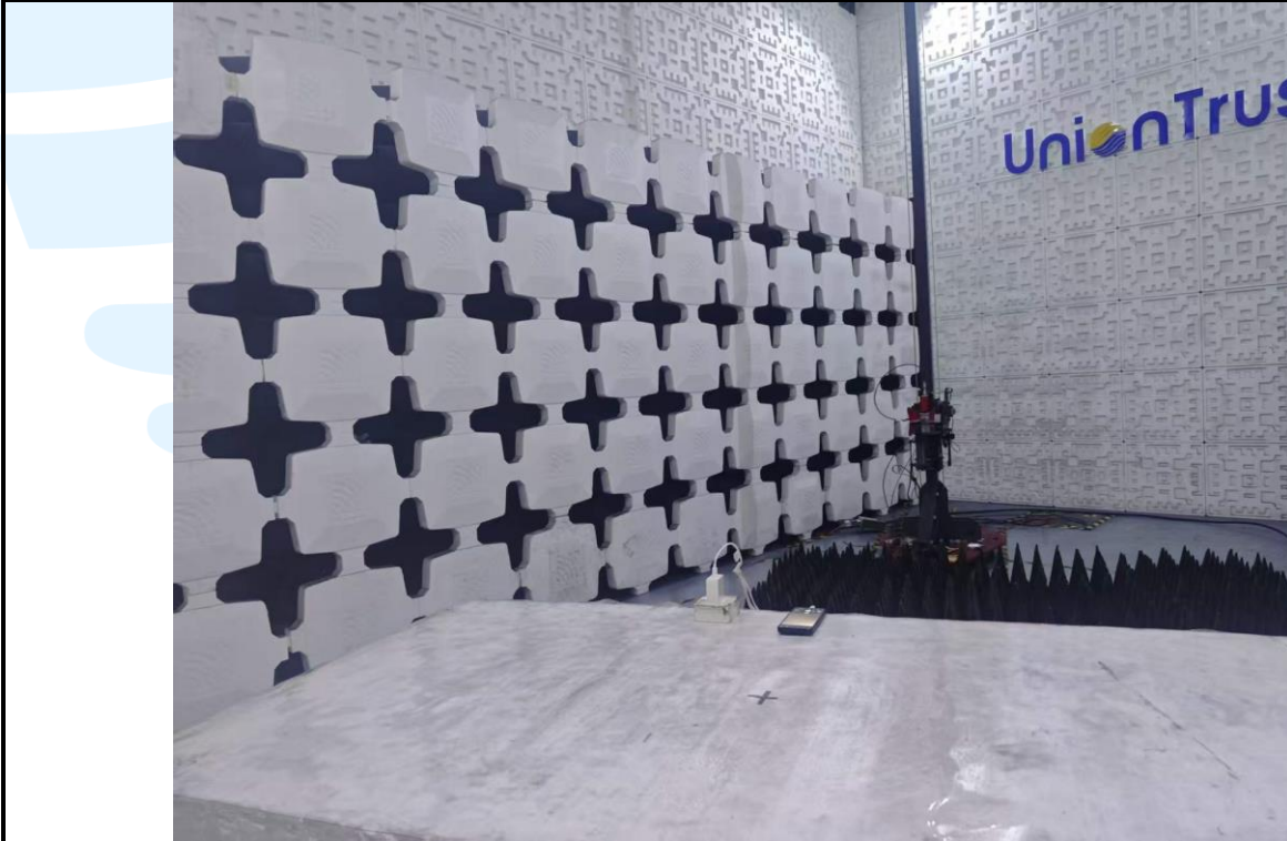
Radiated emission Test Setup (Above 1 GHz) _ Test Mode 2
