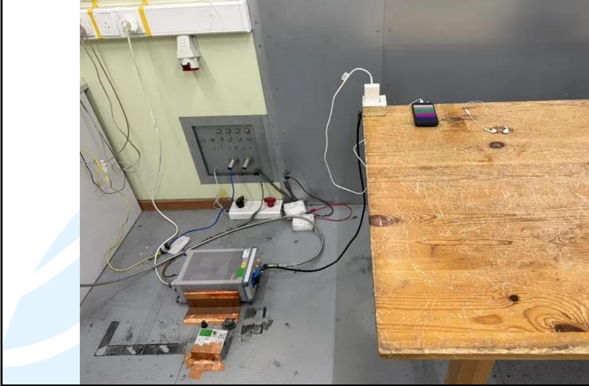
Conducted Emission Test Setup _ Test Mode 1
