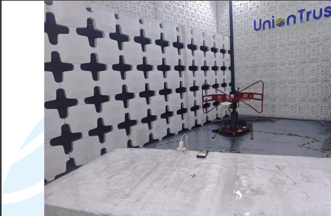
Radiated emission Test Setup (30 MHz~1 GHz) _ Test Mode 2
