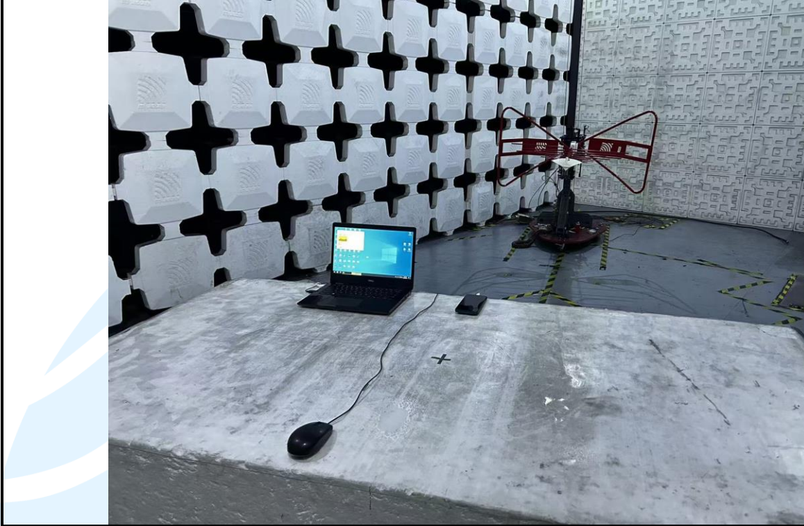
Radiated emission Test Setup (30 MHz~1 GHz) _ Test Mode 7
