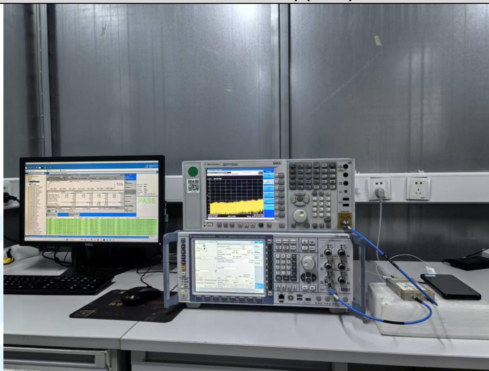
RF Conducted Test Setup (2/3/4G)
