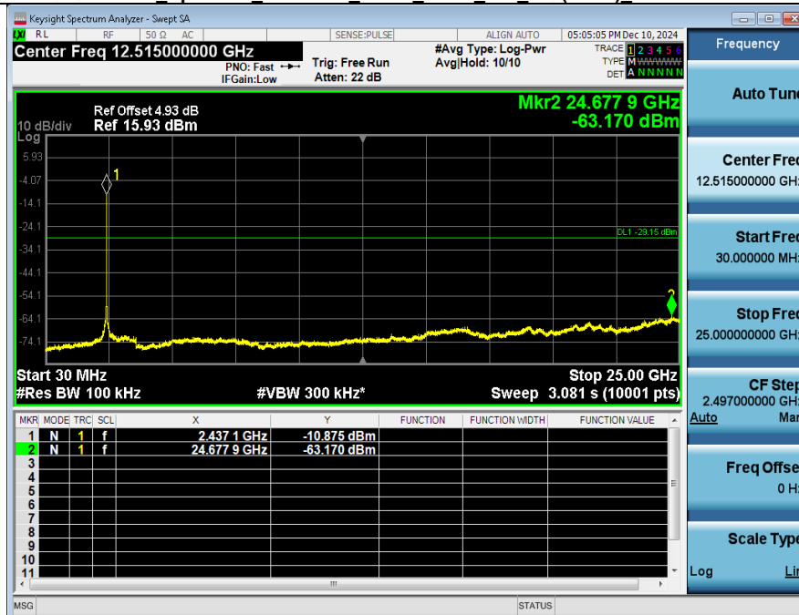
2 Spurious Emission_NVNT_ANT2_802_11n(HT20)_2437
