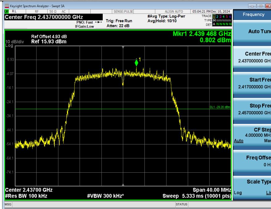
2 Spurious Emission_NVNT_ANT1_802_11n(HT20)_2437
