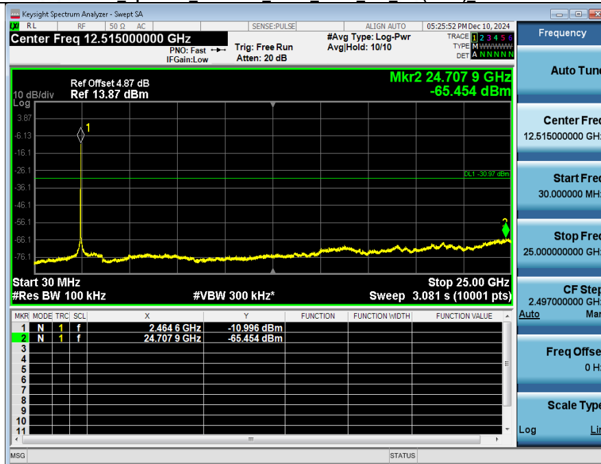
2 Spurious Emission_NVNT_ANT2_802_11n(HT20)_2462
