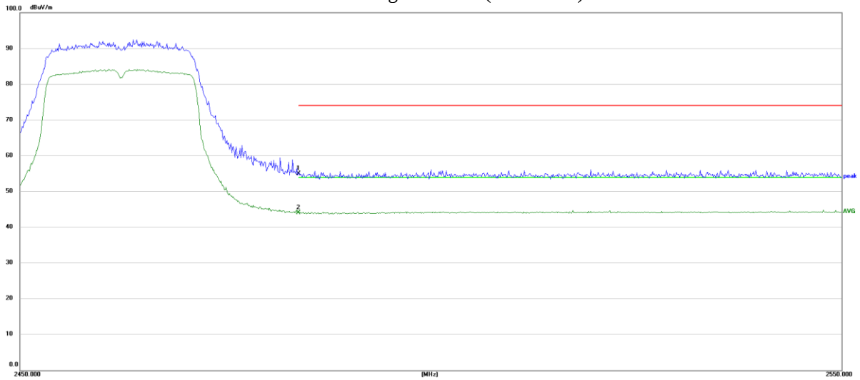
802.11n20 Horizontal High Channel (2462 MHz)-Above 1G
