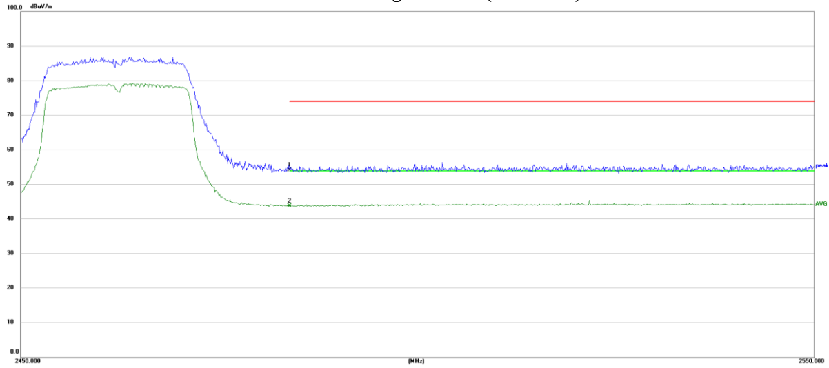
802.11n20 Vertical High Channel (2462 MHz)-Above 1G
