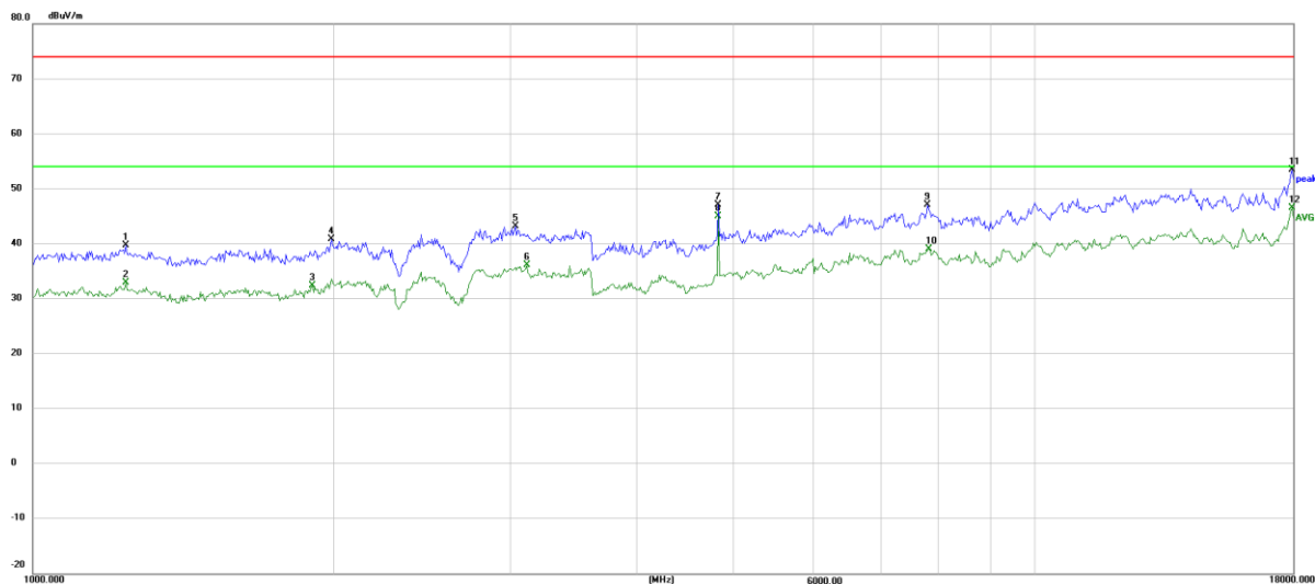
Low Channel (2412 MHz)(802.11b)--Above 1G Vertical
