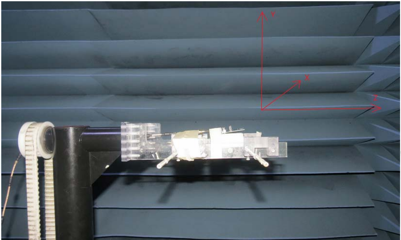
2.4G 3D Gain Picture 2 Test Setup
