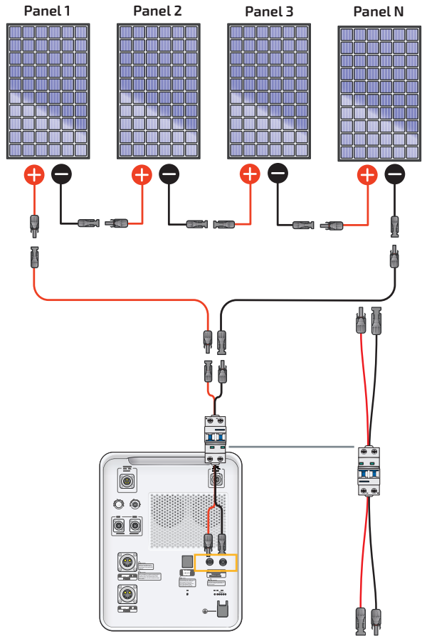
Fig. 5.8 Single unit - PV input port and cable (N panels)
