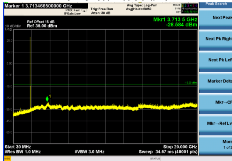
GPRS 1900 Middle channel
