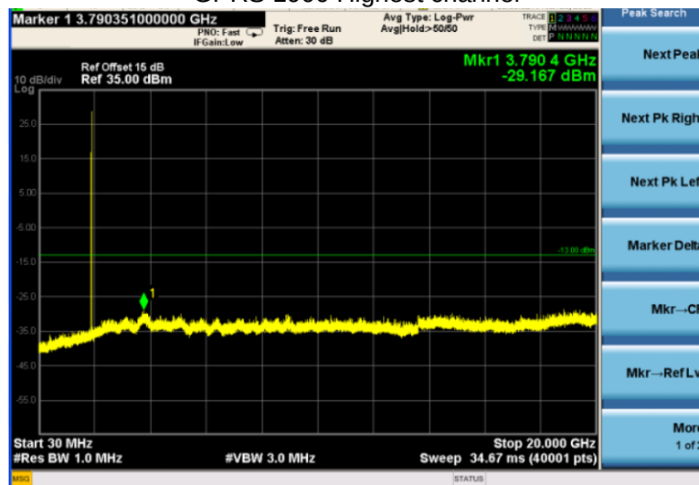
GPRS 1900 Highest channel
