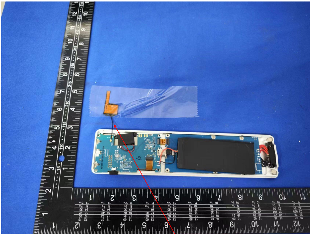
Internal antenna
