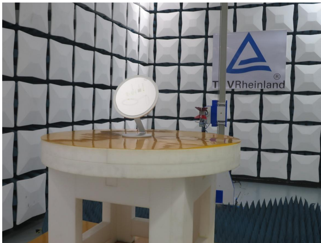
Photograph 2: Set-up photo for Radiated Spurious Emission, 1- 18GHz
