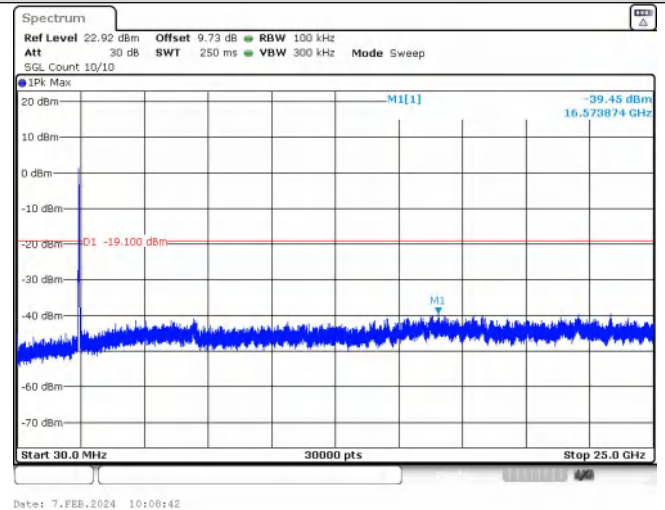
Spurious Emission IEEE 802.11ax_Channel 9_40MHz_Antenna 0_RU&Index SU
