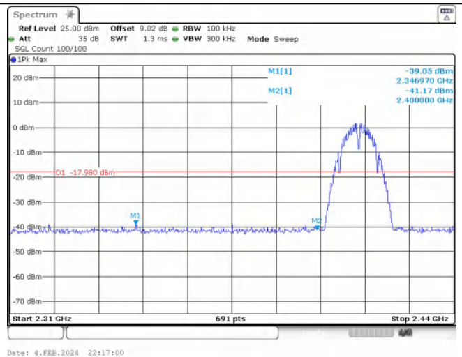
Out Of Band Emission IEEE 802.11b_Channel 1_20MHz_Antenna 0
