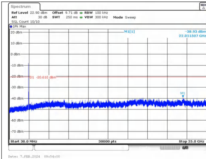
Spurious Emissions IEEE 802.11ax_Channel 6_20MHz_Antenna 0_RU&Index SU
