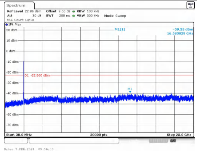
Spurious Emission IEEE 802.11ax_Channel 11_20MHz_Antenna 0_RU&Index SU
