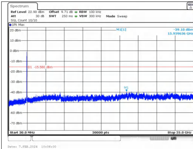
Spurious Emissions IEEE 802.11ax_Channel 6_40MHz_Antenna 0_RU&Index SU
